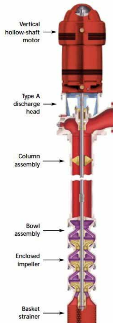
Typical vertical turbine pump profile
